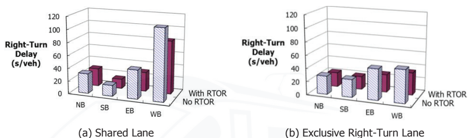
Exhibit 31-59 Effect of Right-Turn-on-Red and Lane Allocation on Delay
